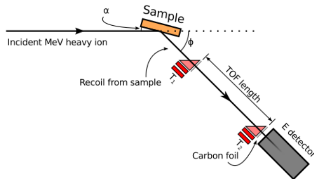
Figure 3.1: Basic setup of recoil spectrometer
